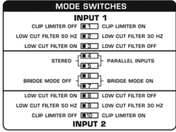
Fig 2.3: DIP-switches
